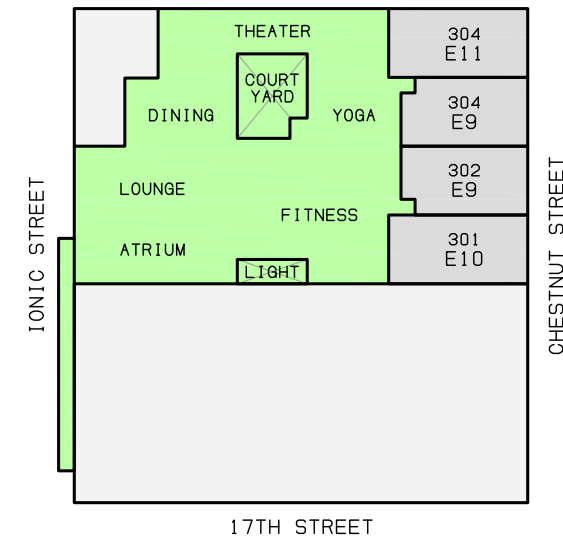
3RD FLOOR
