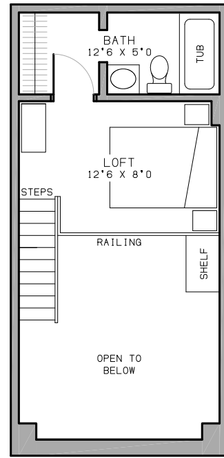
LOFT LEVEL
